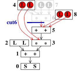
(h) Subgraph 6
