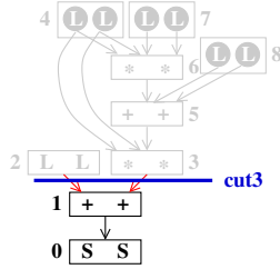
(e) Subgraph 3
