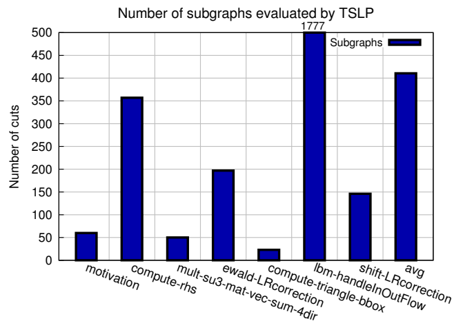
Figure 7. The total number of subgraphs explored by TSLP. Each subgraph corresponds to a cut of the SLP graph.
