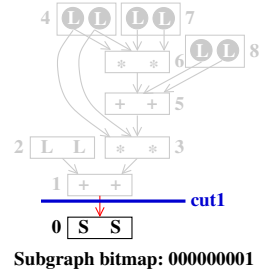
(c) Subgraph 1
