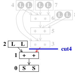
(f) Subgraph 4
