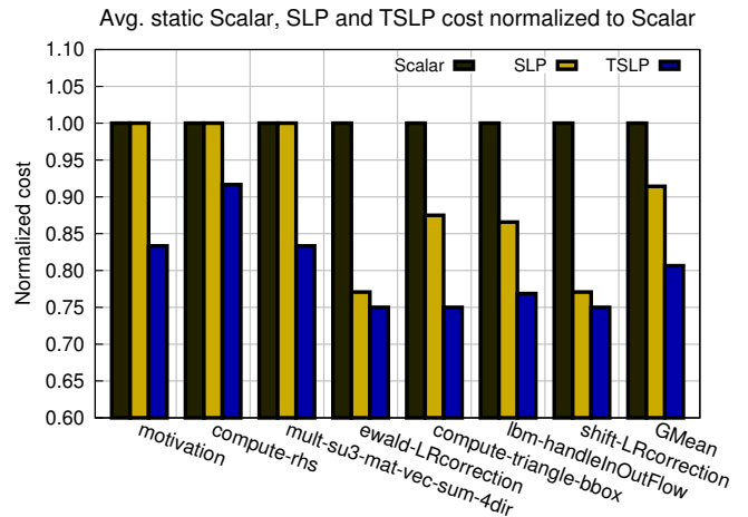
Figure 6. Static cost of Scalar, SLP and TSLP normalized to the scalar cost of the region.
