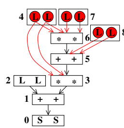
(b) Example TSLP graph
