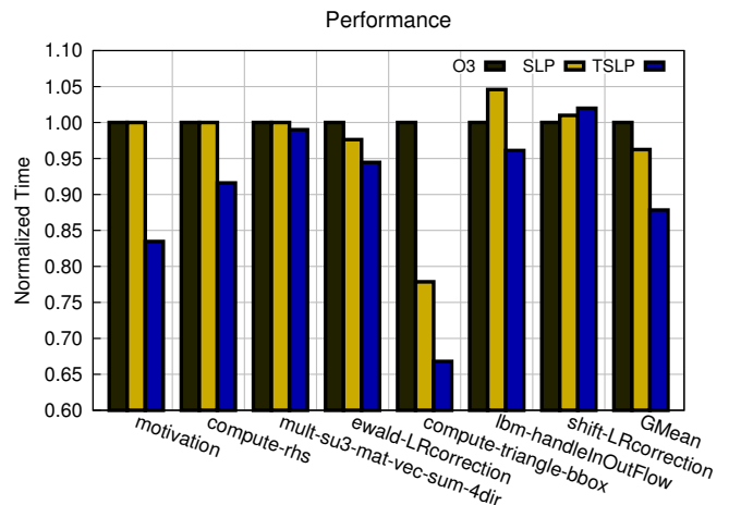
Figure 5. Execution time of the kernels under O3, SLP and TSLP, normalized to the baseline O3.
